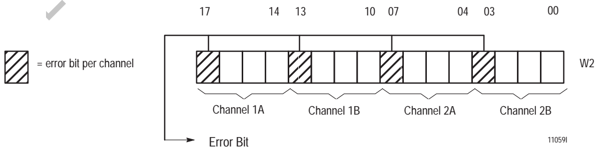
Figure 5.7 Second Auxiliary Diagnostics/Status Word
