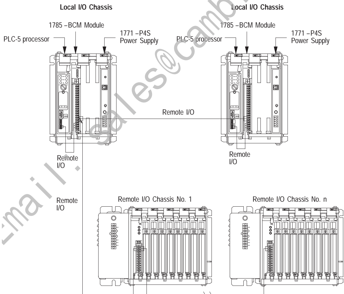
Figure 3.7 Remote I/O Connections
