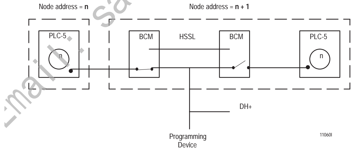
Figure 5.8 Access Point to the Secondary Processor (DH+)
