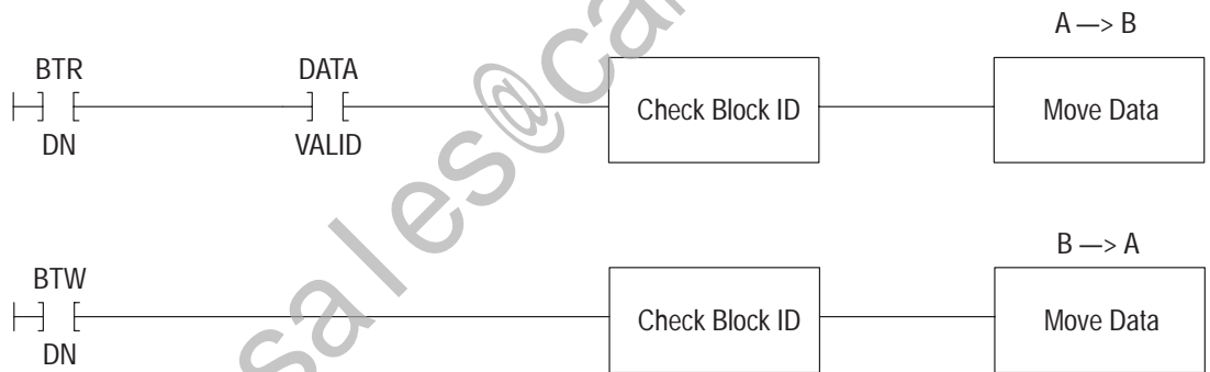
Figure 6.3 Typical Data Move Rungs
