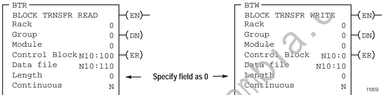
Figure 5.3 Block Transfer Instructions
