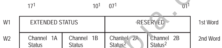
Figure 5.6 Auxiliary Diagnostics/Status Words
