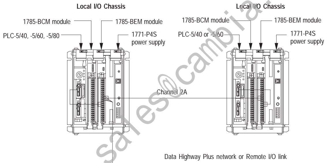
Figure 4.8 Channel 2A Connections
