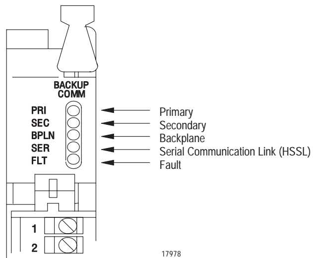
Figure 2.1 1785-BCM Module Status Indicators
